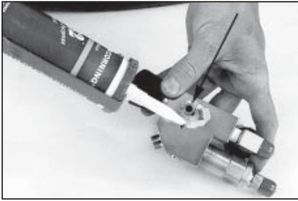
Fig. 6.30 The silicone sealant must not to block the air tube opening.
