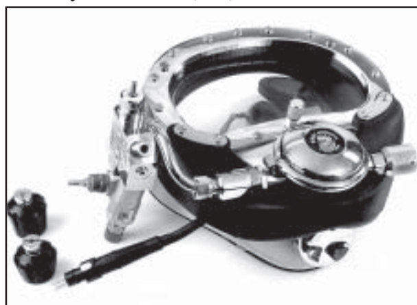
Fig. 7.1 Remove the auxiliary valve and free flow knobs to install the hot water shroud.
